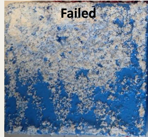
Efflorescence Test
